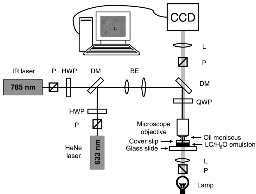
FIGURE 1 Experimental apparatus, P: polarizer, HWP: half-wave plate, DM: dichroic mirror, L: lens, CCD: ccd camera, BE: beam expander for objective back aperture overfilling, QWP: quarter-wave plate (for the appropriate laser wavelength).
