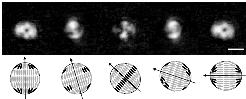
FIGURE 2 Upper panel: sequence of frames of an acquired movie showing a nematic liquid crystal micrometric droplet observed between crossed polarizers, during its laser-induced rotation. Scale bar: 1\text{ }\mu\text{m} . The polarizers axes were oriented at about \pm 45^\circ from the figure vertical direction. Lower panel: schematic representation of the corresponding molecular director configuration occurring within the droplet, as deduced from the crossed-polarizer images (black ellipsoids correspond to regions in which the molecular director is roughly aligned with the polarizer axes and light is blocked). The only region of the droplet in which the dark (crossed) regions are not well explained by our simple graphical analysis is its centre, possibly because of some director reorientation induced by the optical torque itself.
