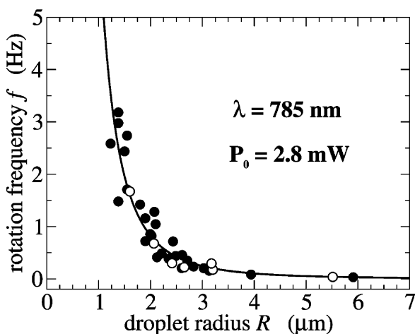
FIGURE 3 Frequency of droplet rotation induced by circularly polarized IR light having a wavelength that falls outside the dye absorption band, for the case of dye-doped (filled circles) and pure (open circles) liquid crystal, as a function of droplet radius. The laser power on the sample was 2.8 mW. The solid line is a theoretical prediction based on the model reported in the text.
