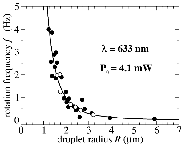
FIGURE 4 Frequency of droplet rotation induced by circularly polarized light from a He-Ne laser, which is absorbed by the dye, for the case of dye-doped (filled circles) and pure (open circles) liquid crystal, as a function of droplet radius. The laser power on the sample was 4.1 mW. The solid line is a theoretical prediction based on the model reported in the text.
